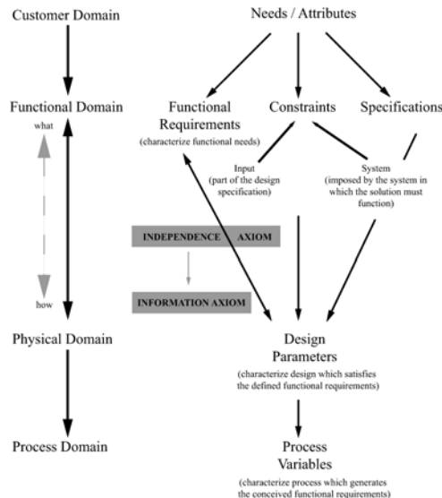
Figure 2 Axiomatic design process according to N. P. Suh. The design process is iterative in a sense that the process is not linear and the designer switches between the domains (Suh, 2001)
