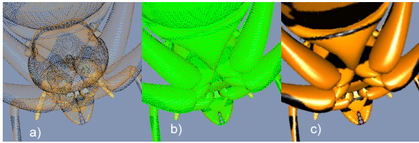
Figure 12: Hole detection and image reconstruction. a) Surfel object with holes. b) Hole detection (hole pixels in green). c) Image reconstruction with a Gaussian filter.
