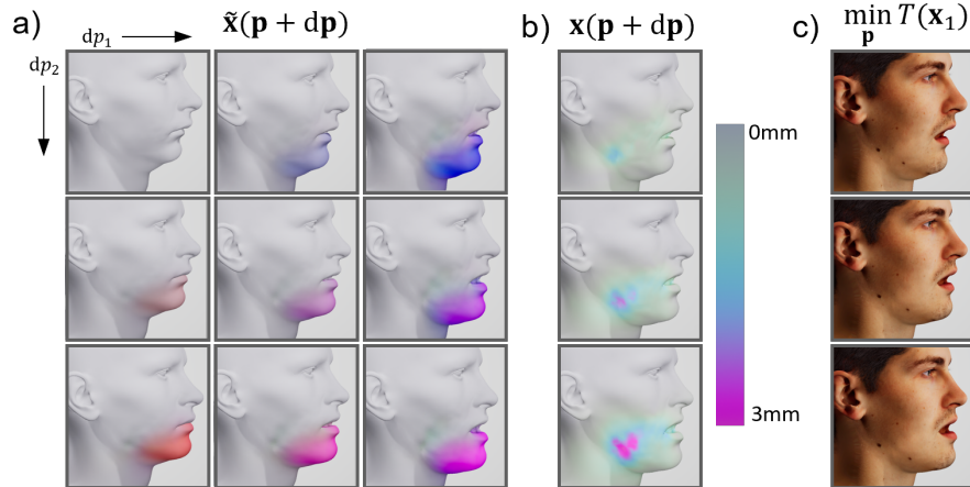
Figure 5: a) Estimated equilibrium state for perturbed dp , showing how increasing one element of p changes the estimate. We vary blendshapes responsible for the downwards and sideways translation of the mandible, and colour the surface displacement in each direction as blue or red respectively. b) True equilibrium state for rightmost column of a), recomputed using forward simulation. Colour shows the estimate's error. c) Optimising p to find a true equilibrium state as close as possible to the predicted \tilde{x} . No error plot was generated, due to the optimal parameters being imperceptibly similar to those from b).
